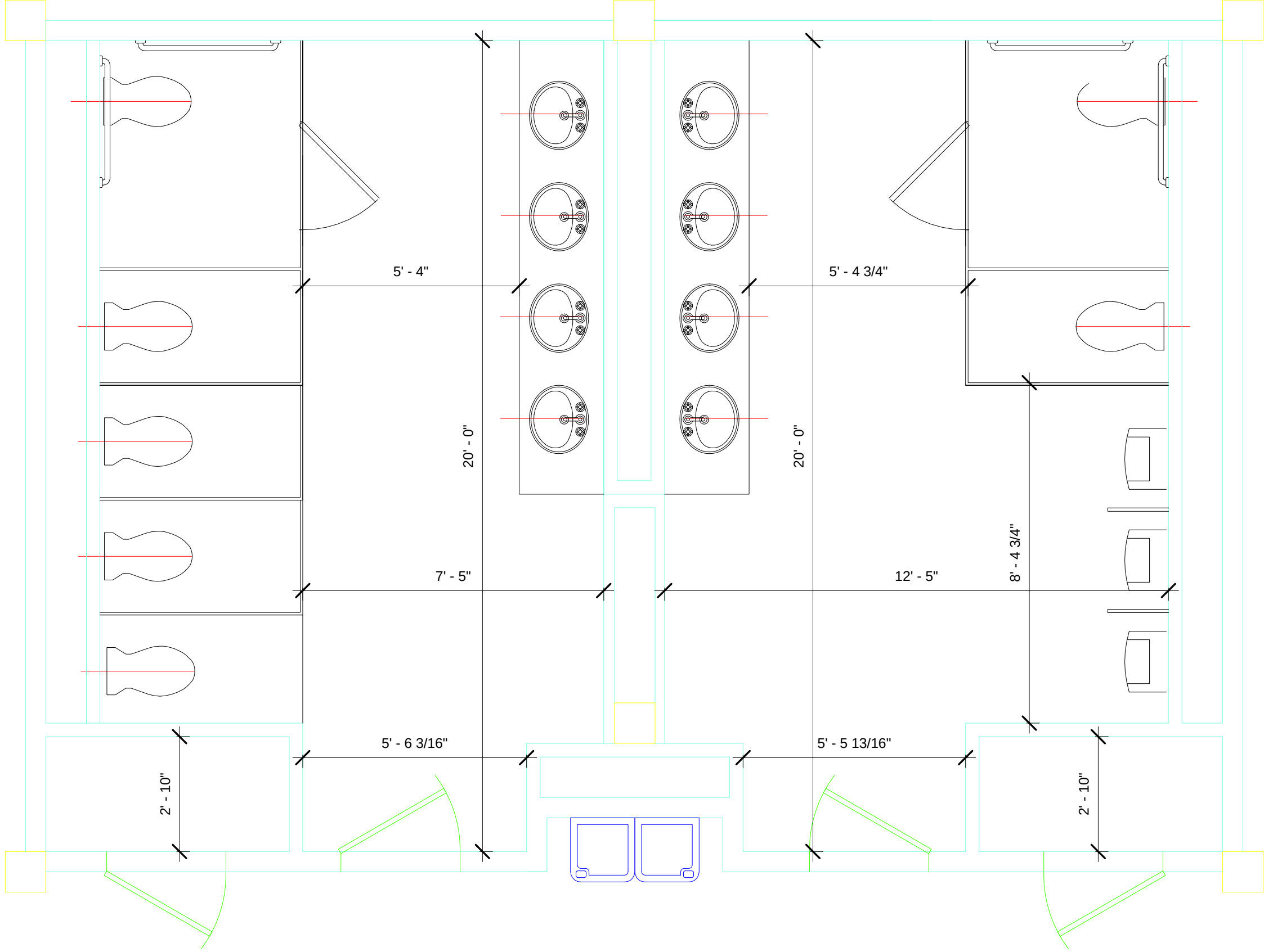
1 FLOOR PLAN (C) 3/8" = 1'-0"
