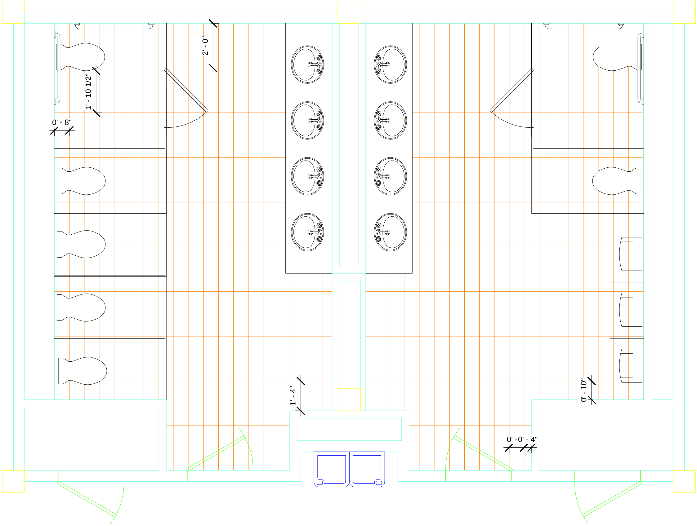
1 FLOOR TILE LAYOUT (C) 3/8" = 1'-0"
