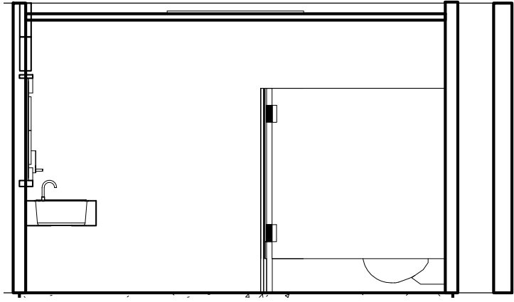
② MENS NORTH ELEVATION 1/4" = 1'-0"
