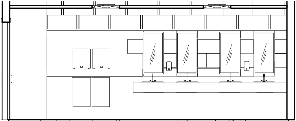
④ MENS WEST ELEVATION 1/4" = 1'-0"
