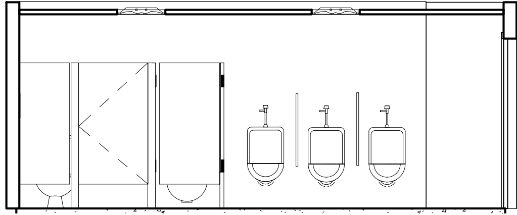
① MENS EAST ELEVATION 1/4" = 1'-0"
