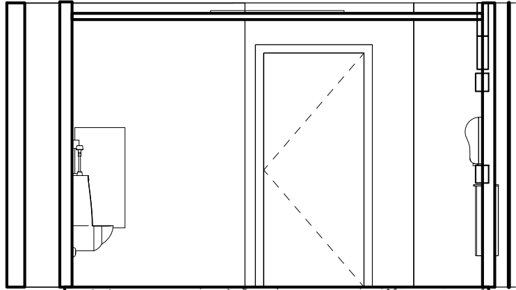
③ MENS SOUTH ELEVATION 1/4" = 1'-0"
